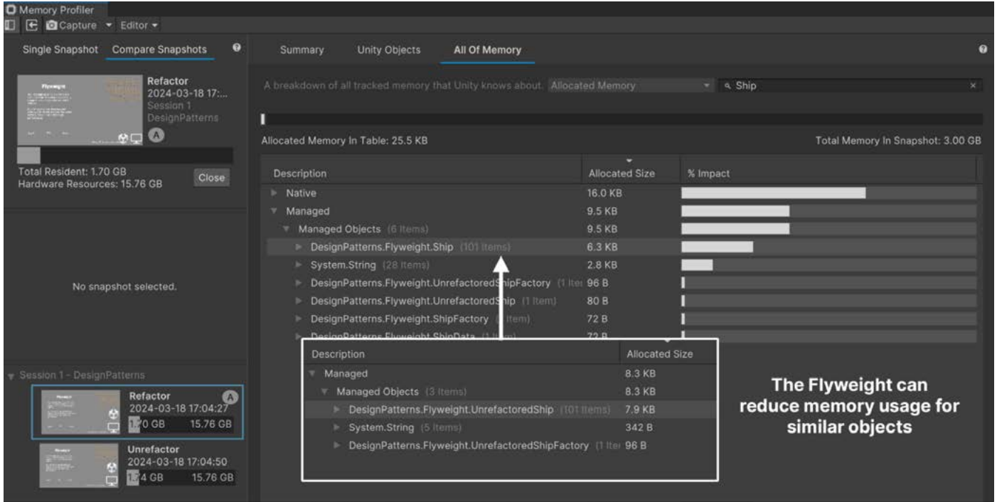
Compare the memory savings in the Memory Profiler.
