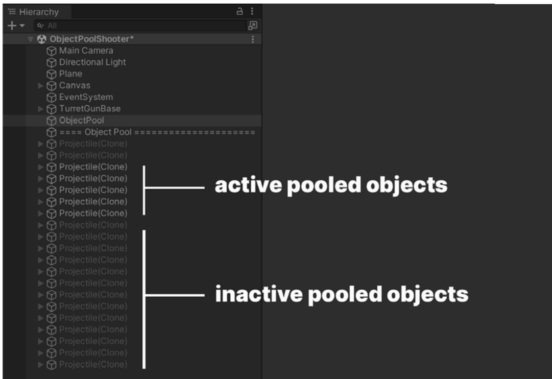
Disable and reuse pooled objects
