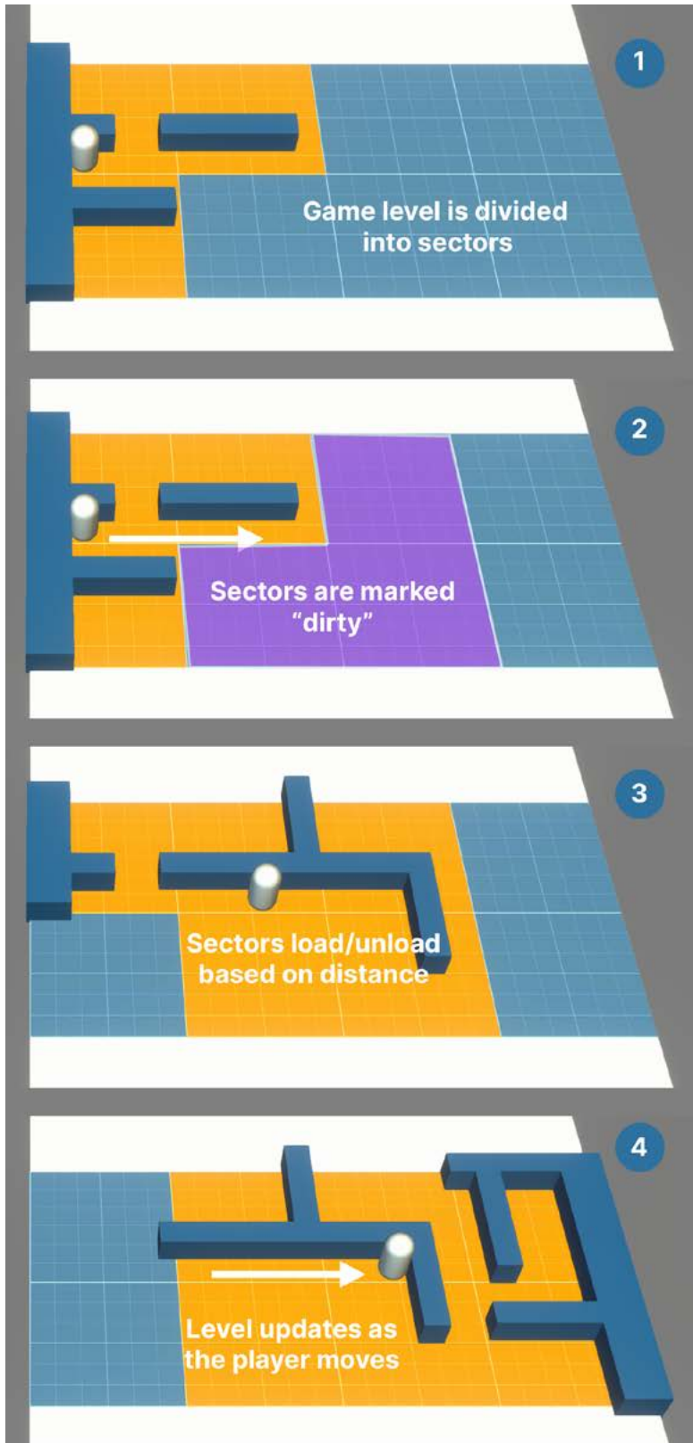
Parts of the level update after they are marked "dirty."
