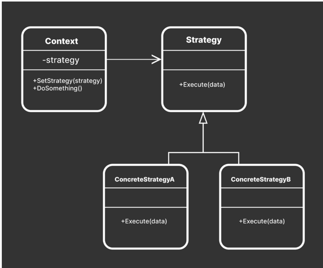
The Strategy pattern makes behaviors interchangeable at runtime.
