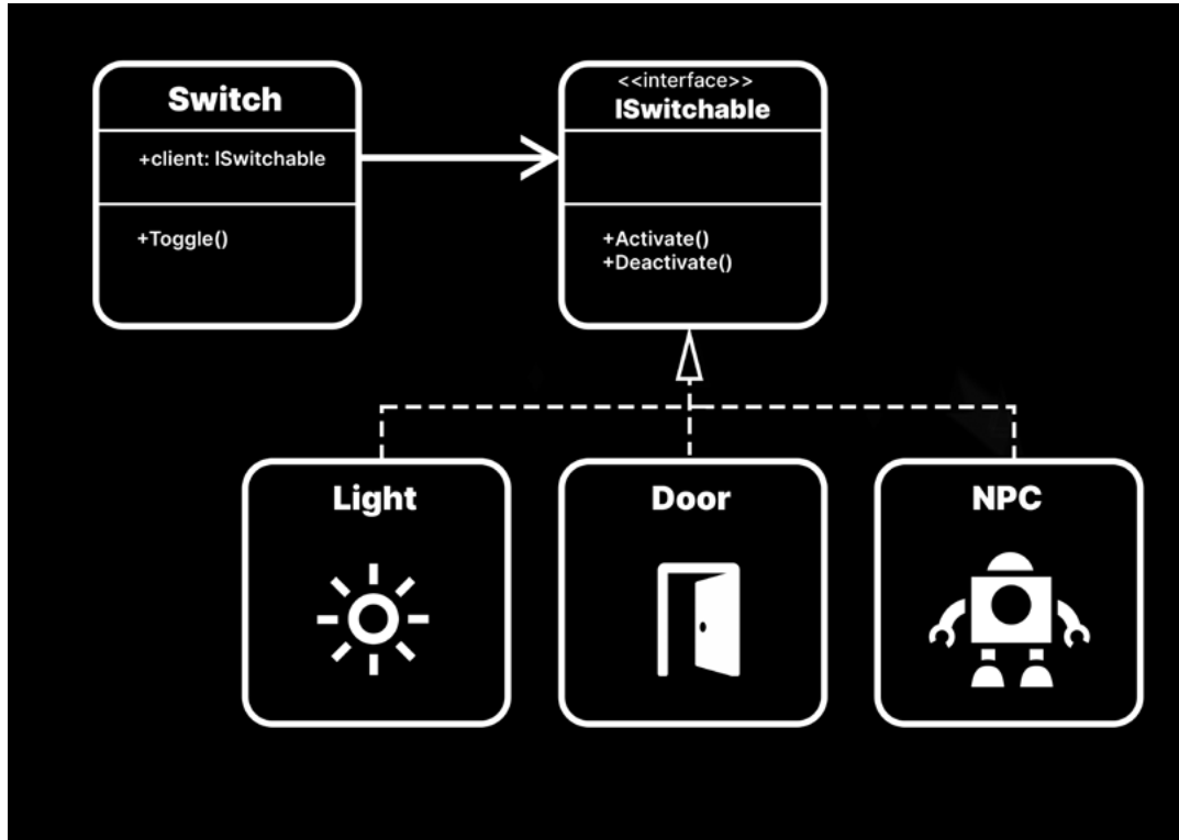
The Switch can now activate any ISwitchable object.
