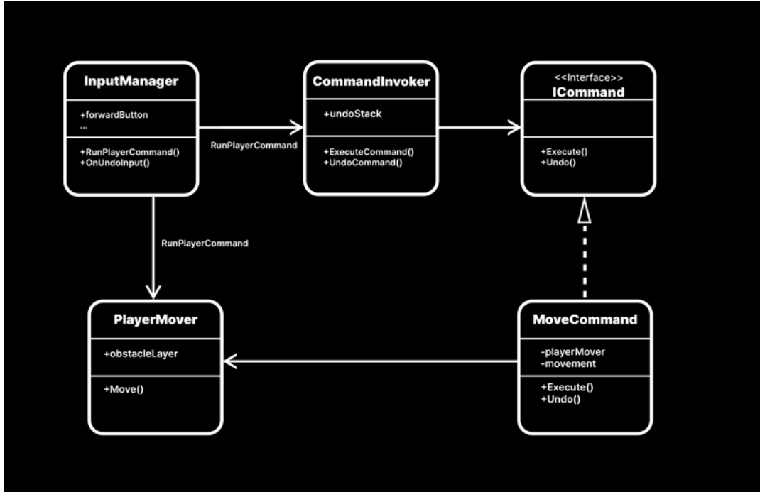
The CommandInvoker, ICommand, and MoveCommand
