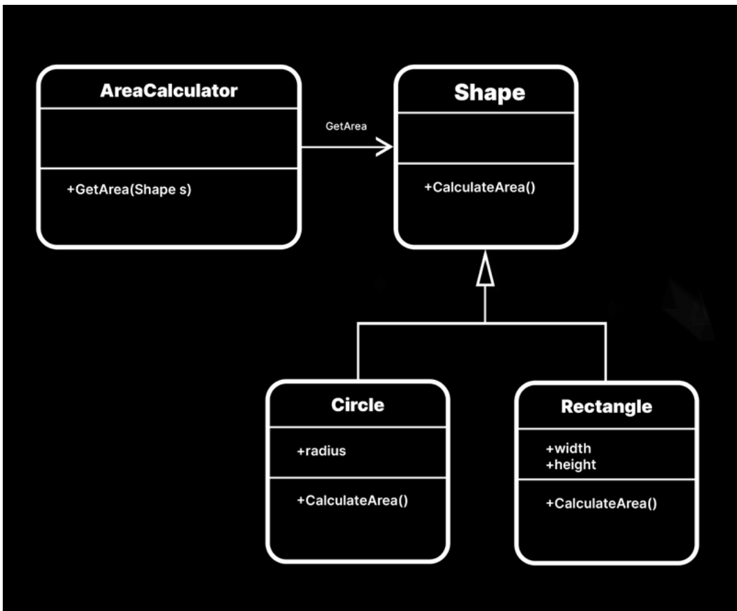
Revising the classes for the open-closed principle
