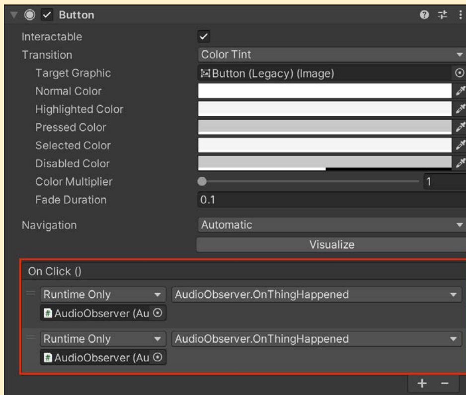
UnityEvents have graphical components for your setup.
