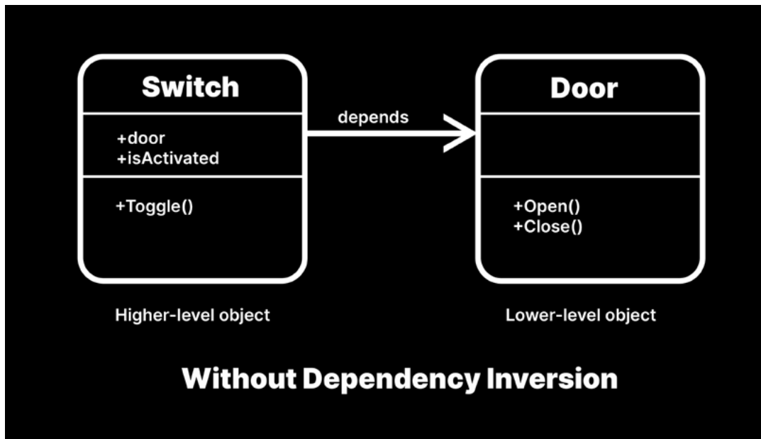
The Switch (high-level) depends directly on the Door (low-level) class.
