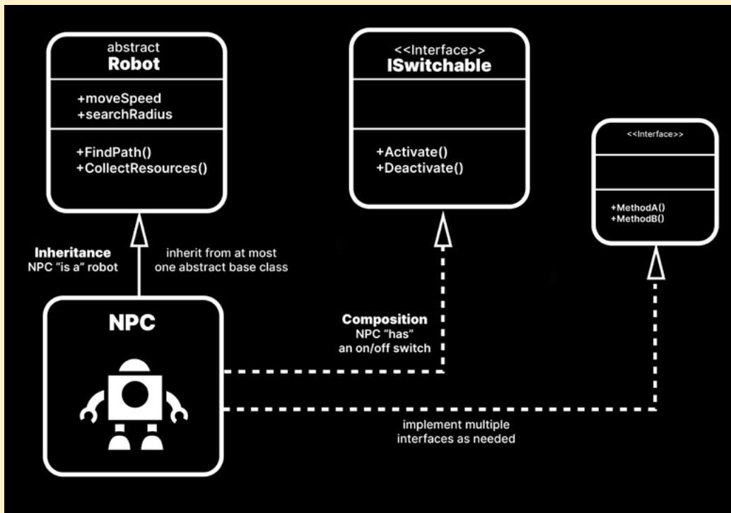
The NPC Robot using both
