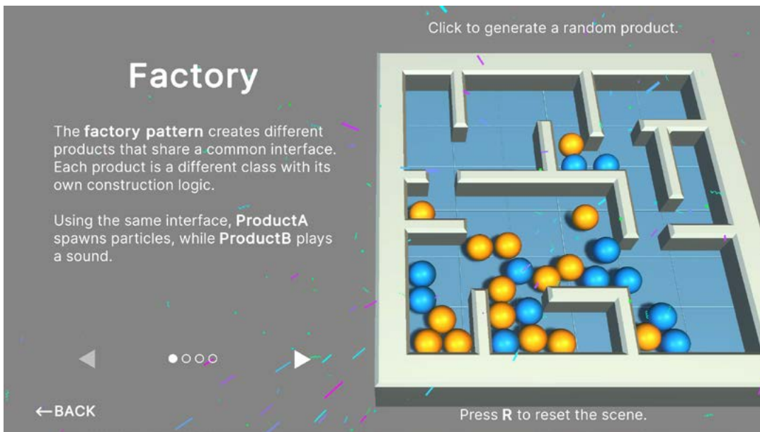
One product plays a sound, while another plays particles. Both use the same interface.
