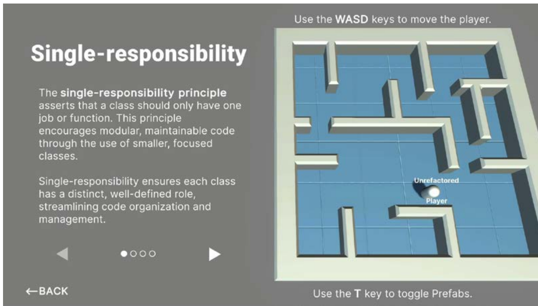
The single responsibility demo separates the Player into smaller components.
