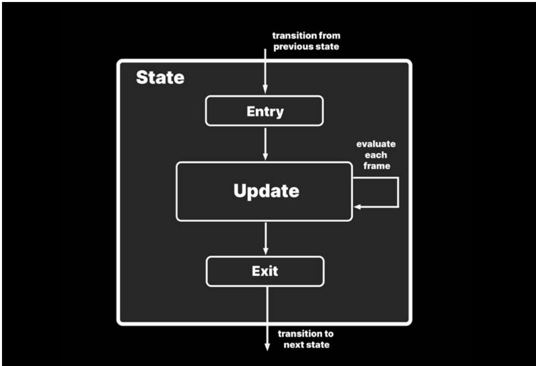
The encapsulated state with an Entry, Exit, and Execute
