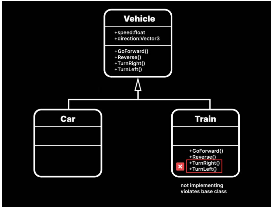
A Train would violate your base class.
