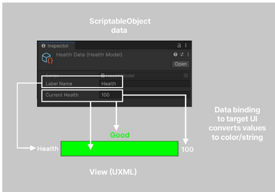
The UI binds to the HealthModel ScriptableObject's values.
