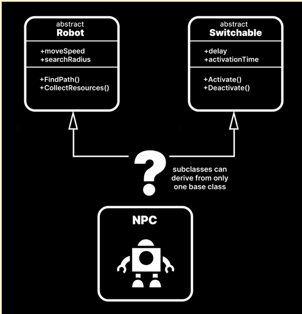
Choosing between base classes
