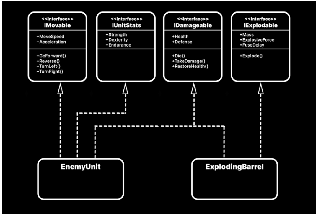
Split the interface into smaller ones.
