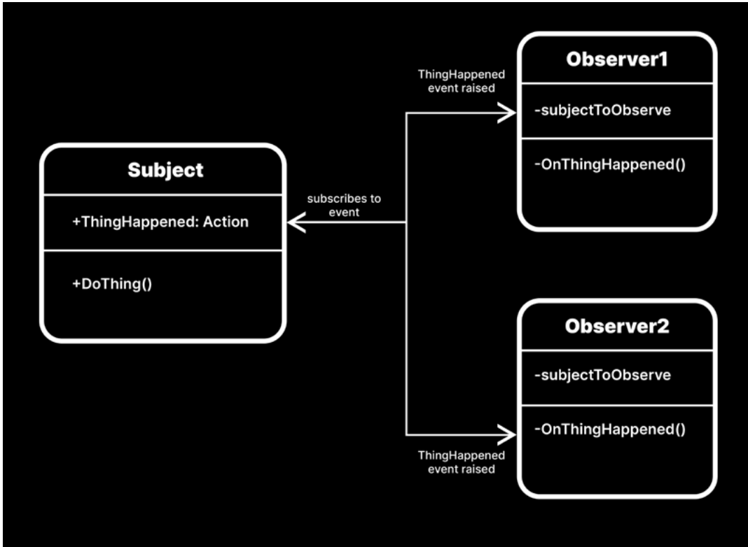
The subject raises the event to notify the observers.
