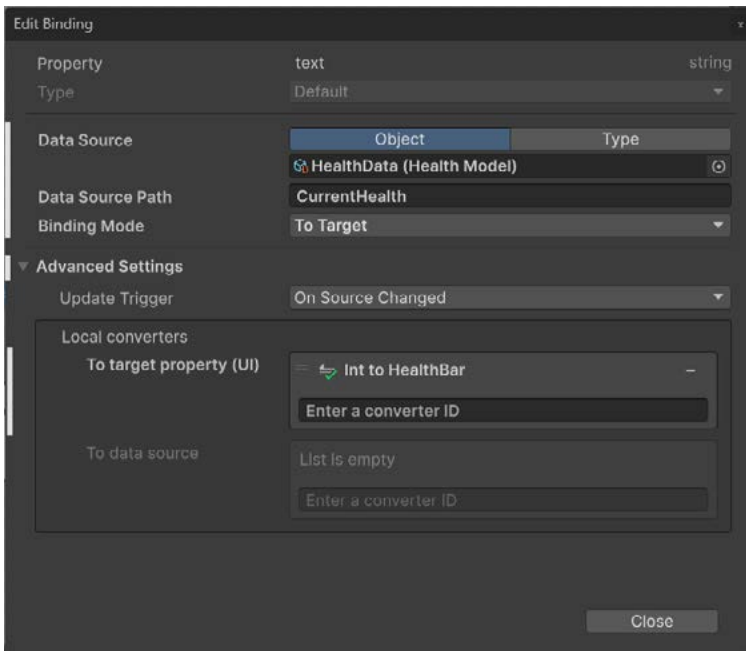
The Edit Binding window.
