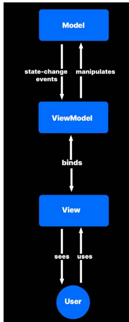
The MVVM pattern.
