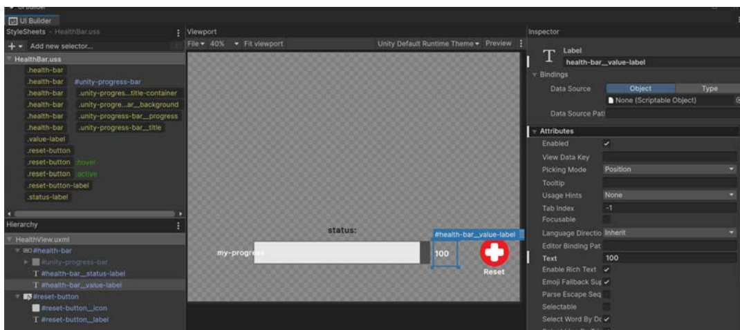
The UXML in the UI Builder
