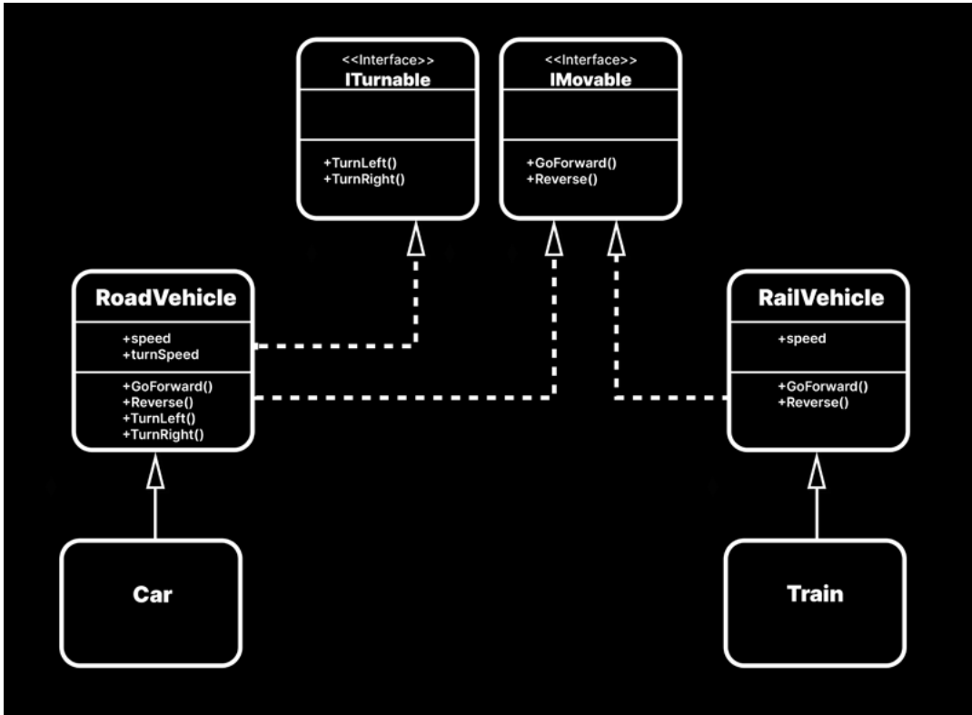
Refactoring to take Liskov substitution into consideration
