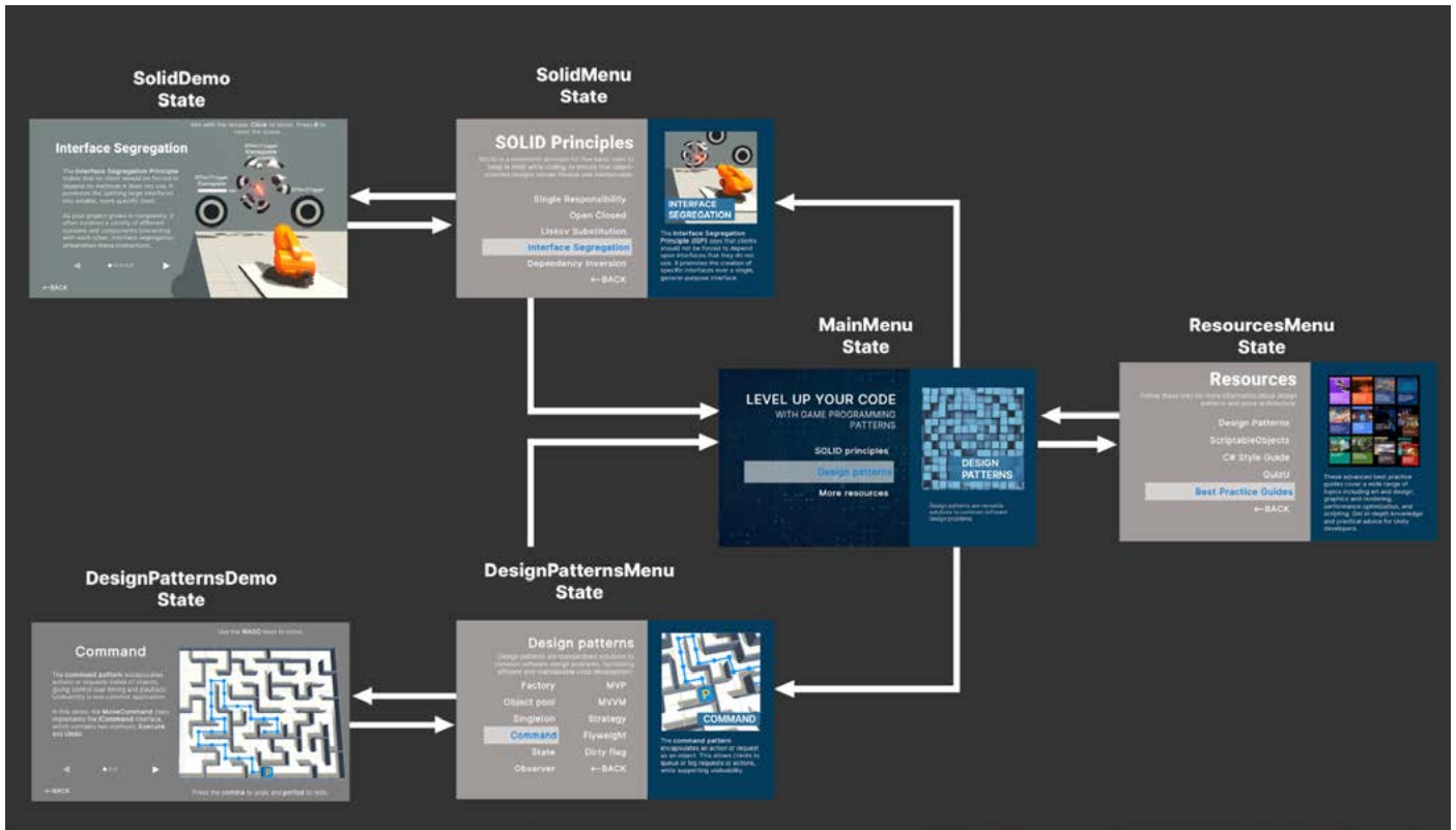
The GameManager state diagram.
