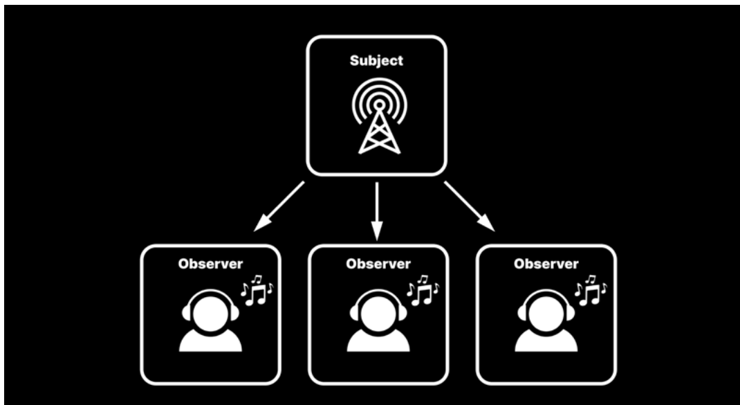
The observer pattern functions like a radio tower. The subject broadcasts to the observers.
