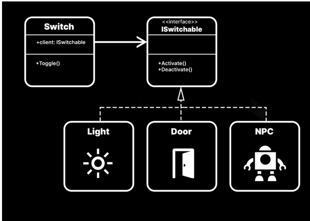
In dependency inversion, high-level modules should not depend on low-level modules. Both depend on abstractions.
