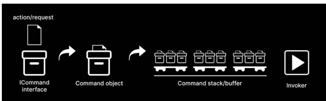
Storing actions with the command pattern
