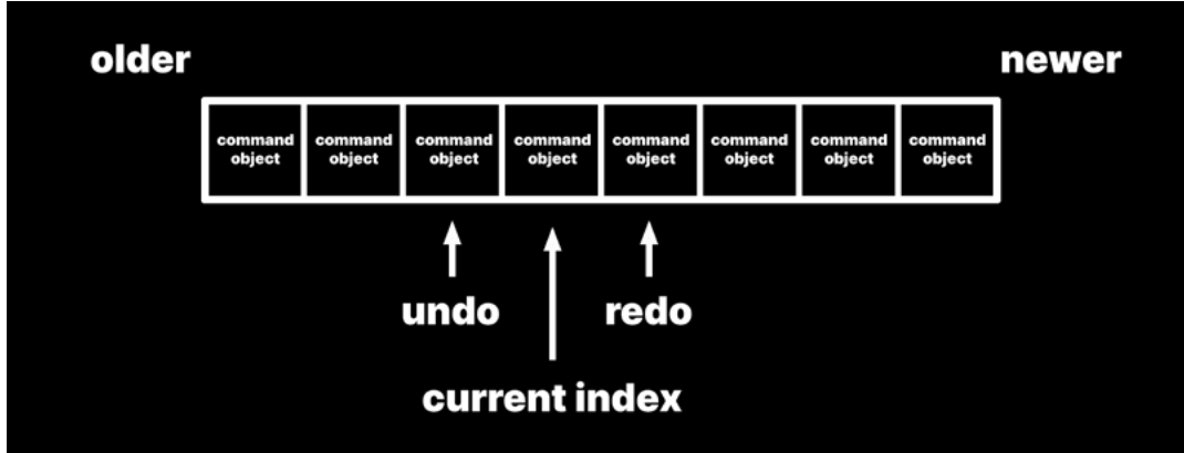
A list or other collection acts as a command buffer.
