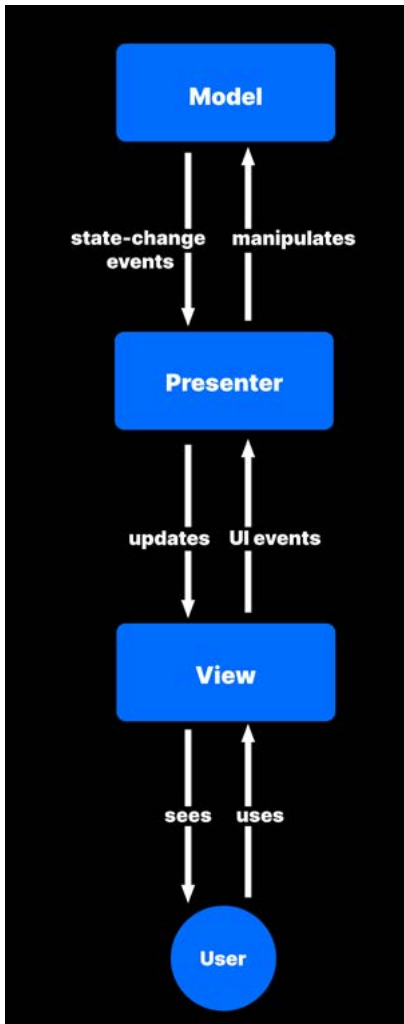
MVP: A variation on MVC
