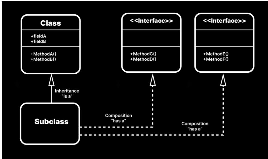
Composition over inheritance
