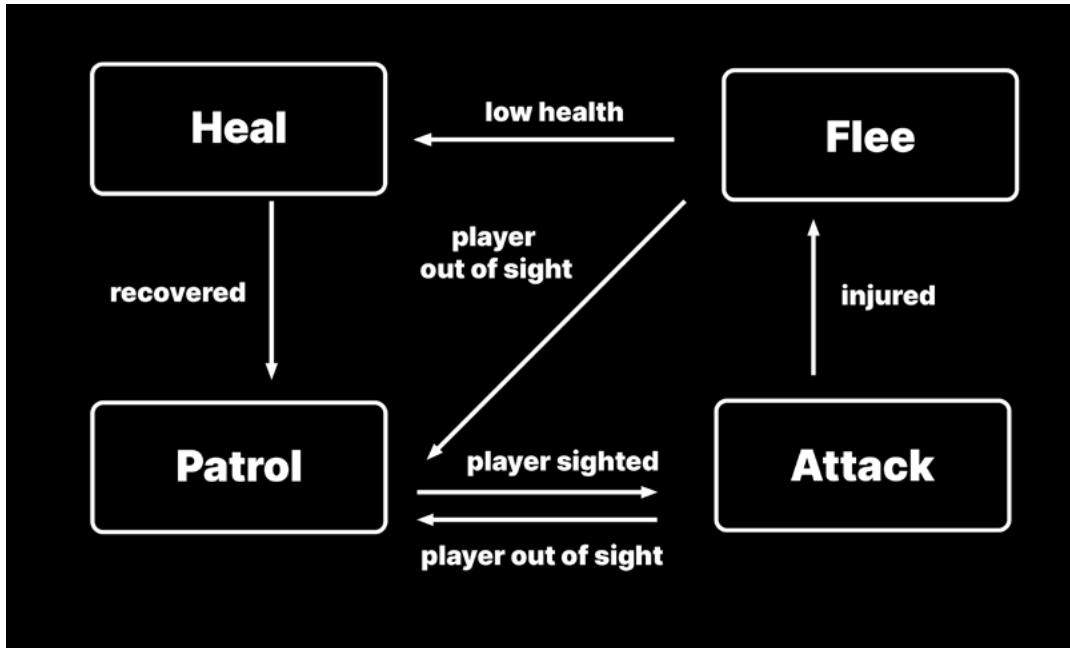
A simple AI based on state patterns
