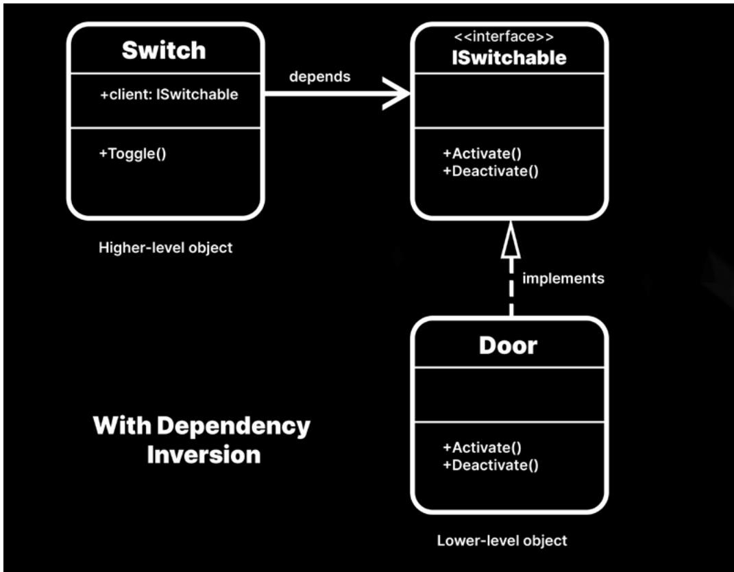
An interface, ISwitchable, between the two classes
