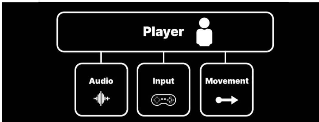
The Player, refactored into classes with single responsibilities
