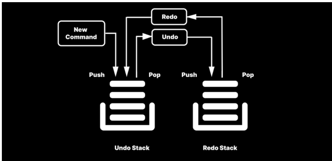
Undo and redo stacks
